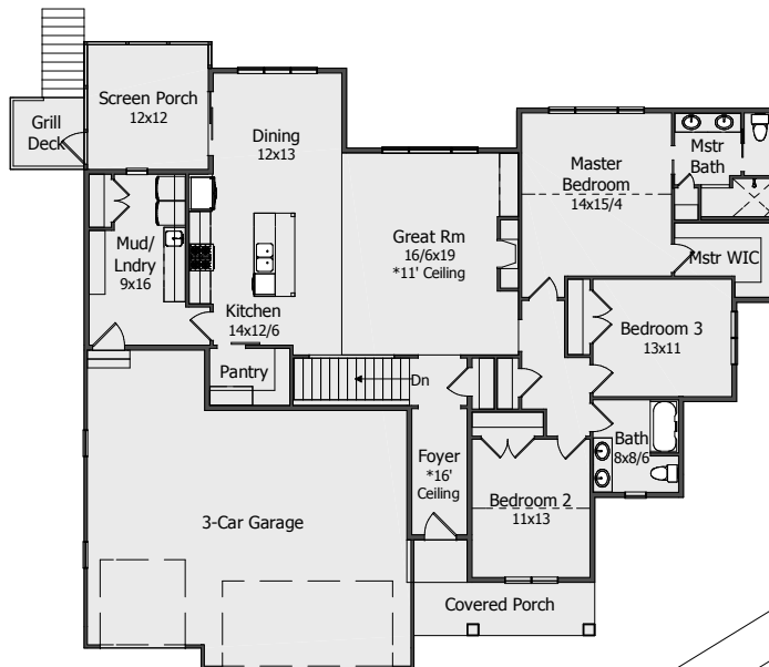
Main Floor 2,000 Sq. Ft.
